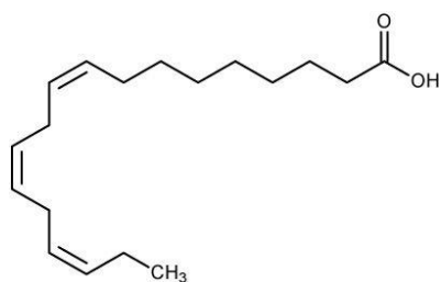
Linolenic acid
